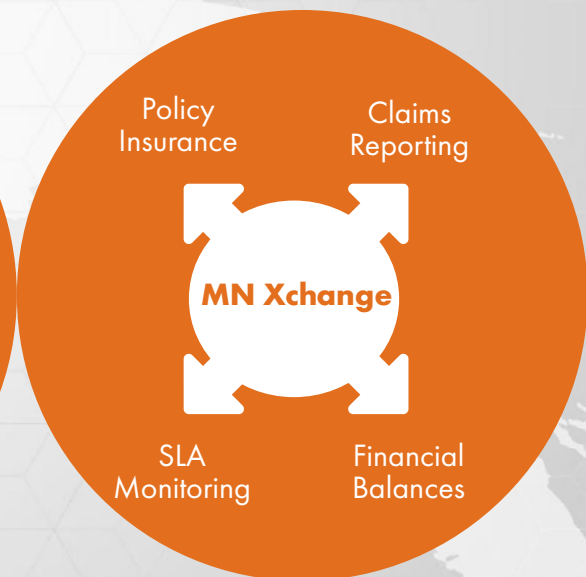
Partner Management
