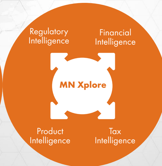
Knowledge Repository
